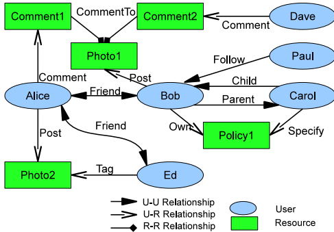
Fig. 3. A Sample Social Graph
