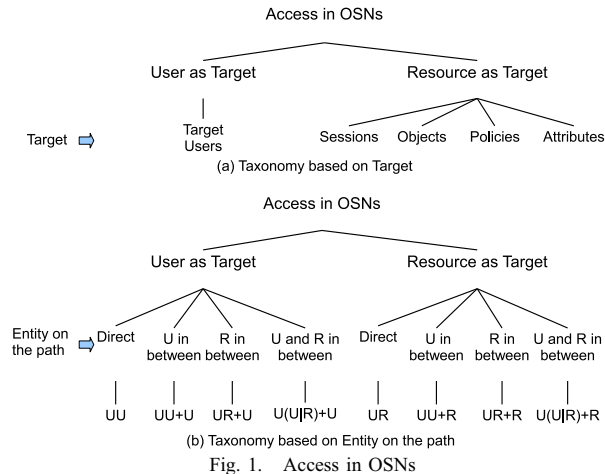
Fig. 1. Access in OSNs
